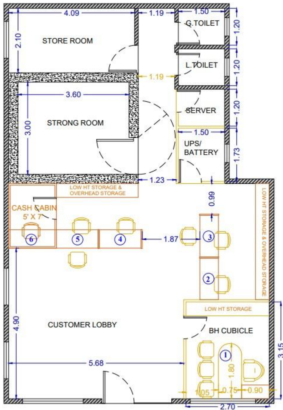
SHELU BAZAR BRANCH- FURNITURE LAYOUT
